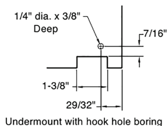
Undermount with hook hole boring
